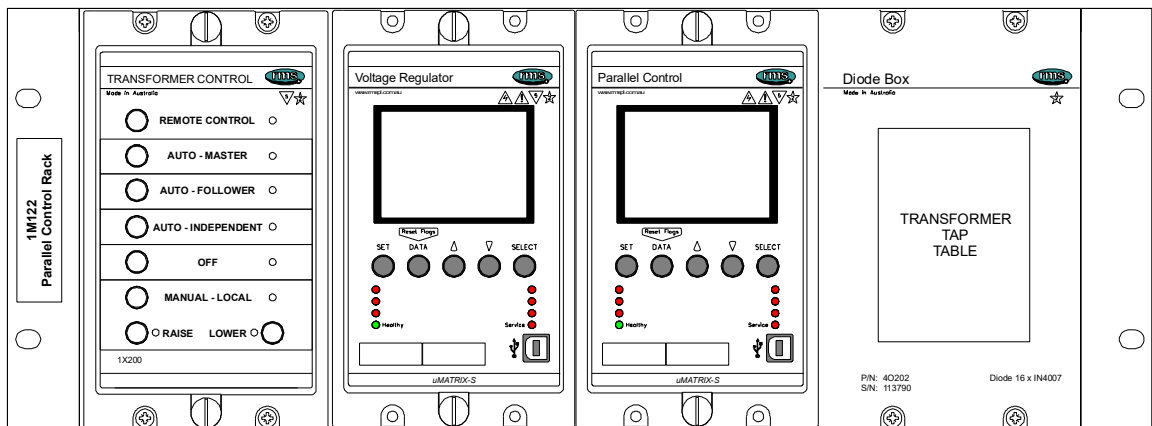
1X200 Transformer Control panel 2V164-S Voltage regulator 2V165-S Parallel Control unit
