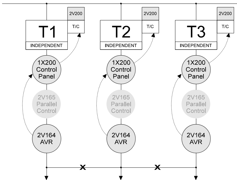
T1, T2 & T3 operating independently No MASTER control selected
