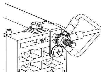
Figure 16: M Series case type earth connection detail
