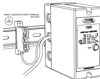
Figure 14: 1S20 DIN rail mount earth connection detail
