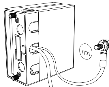
Figure 15: 1S20 panel mount earth connection detail
