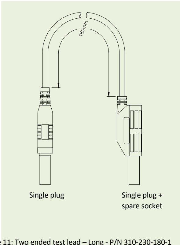
Figure 11: Two ended test lead – Long - P/N 310-230-180-1
