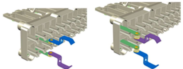
Figure 5: Contact geometry
