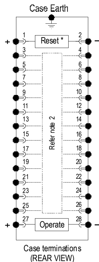
Figure 7: AR12 rear terminal layout
