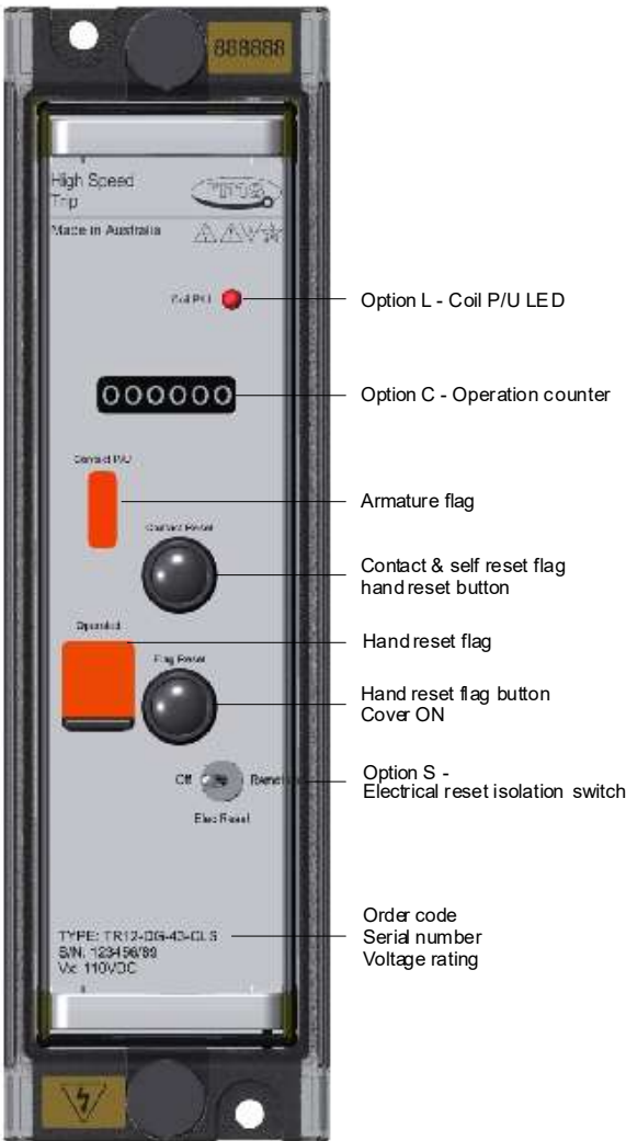
Figure 1: Front panel layout depicting flags, resets & option positions
