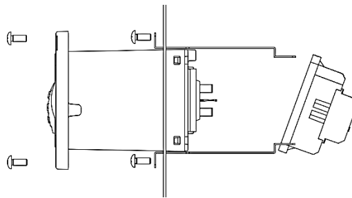
Alternative method for capturing relay base into retention plates
