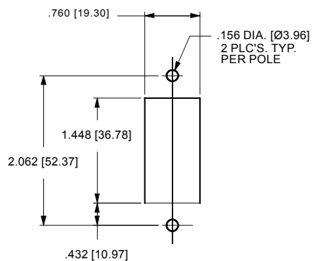
PANEL CUTOUT DETAIL TOLERANCES \pm 0.005 [ .12]
