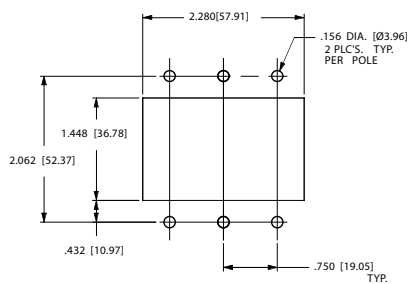
PANEL CUTOUT DETAIL TOLERANCES ±.005 [0.12]
