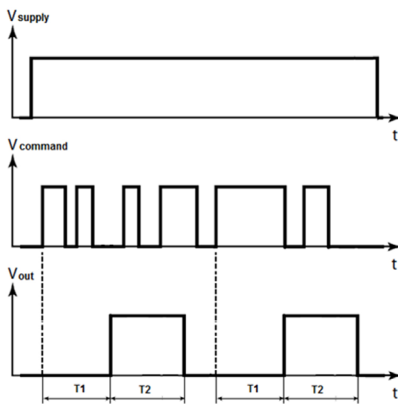
T1 = time delay at pull-in (delay-on), T2 = pulse time. Both T1 and T2 can be adjustable
