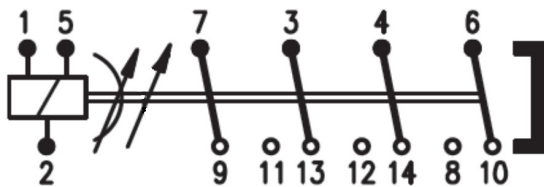
T1 = time delay at pull-in (delay-on), T2 = pulse time. Both T1 and T2 can be adjustable
