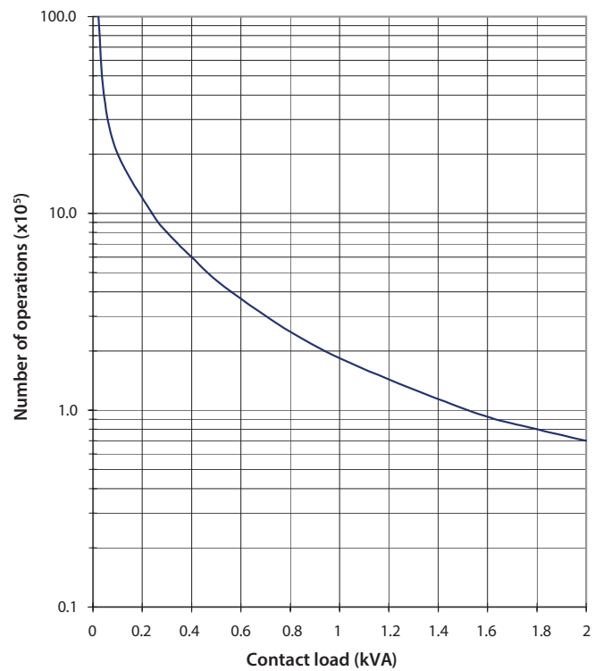
Contact life for resistive AC load single contact
