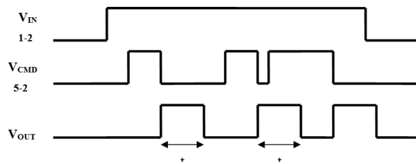
F2- Pulse when command voltage disappears
