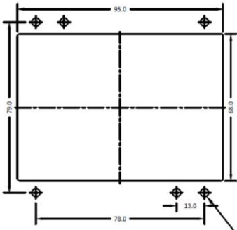
Panel cut-out to flush mount relay with rear connect socket.
