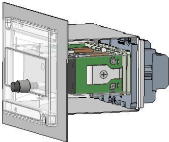
Panel cut-out to flush mount relay with rear connect socket.
